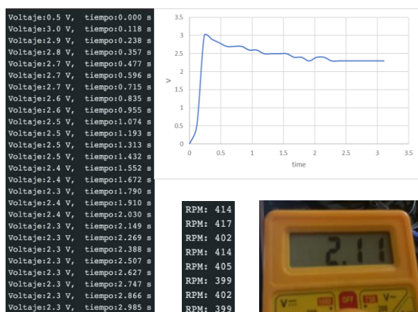
Figure 4. Measured voltage function of time: numerical data and plotted voltage curve.
