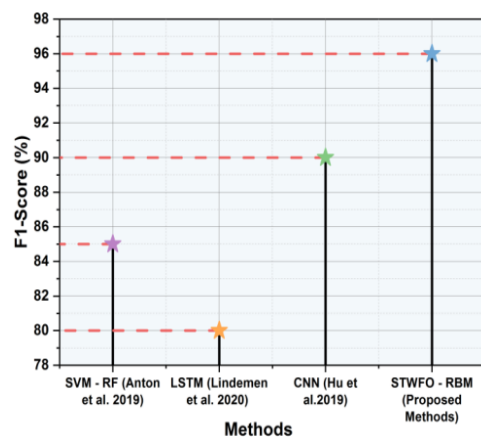
Figure 5. Performance analyses of F1 score.
