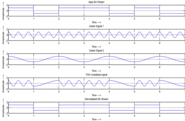
Figure 2. Frequency shift keying modulation and demodulation
